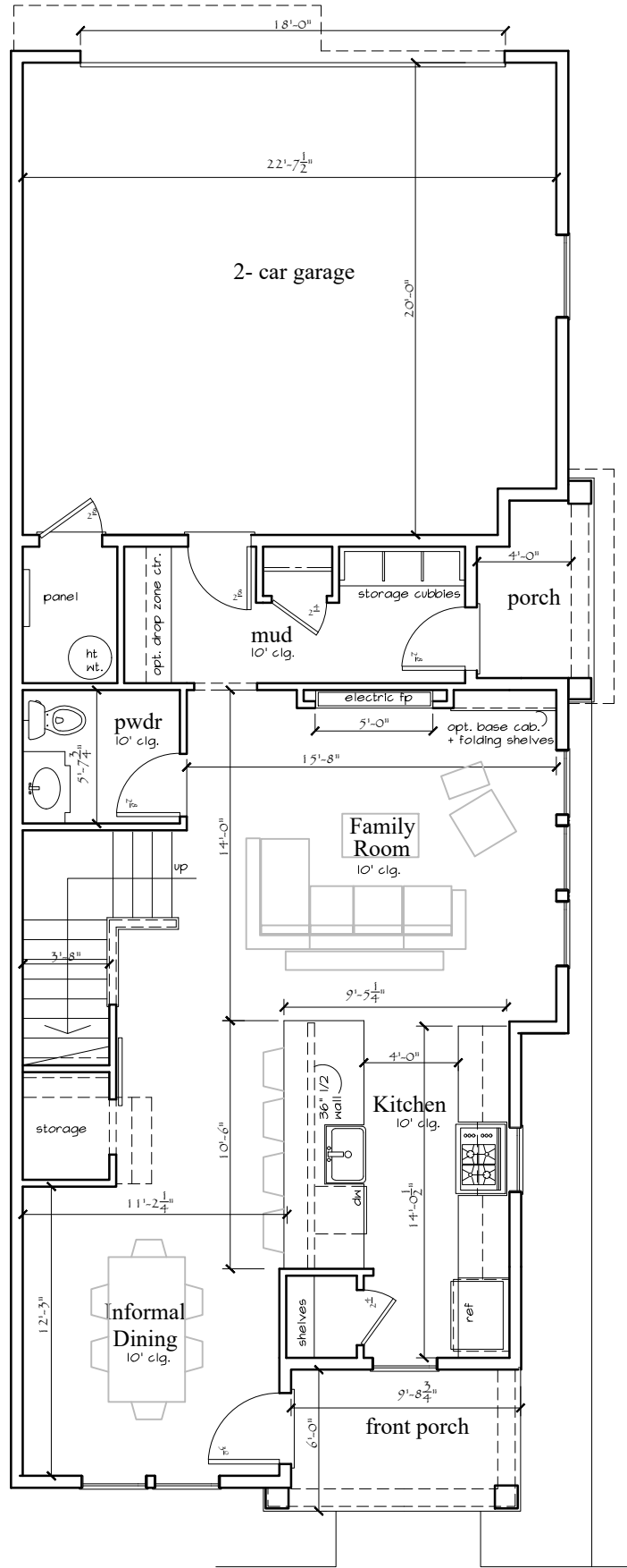
First Floor Plan first floor living opt. 887 s.f.
